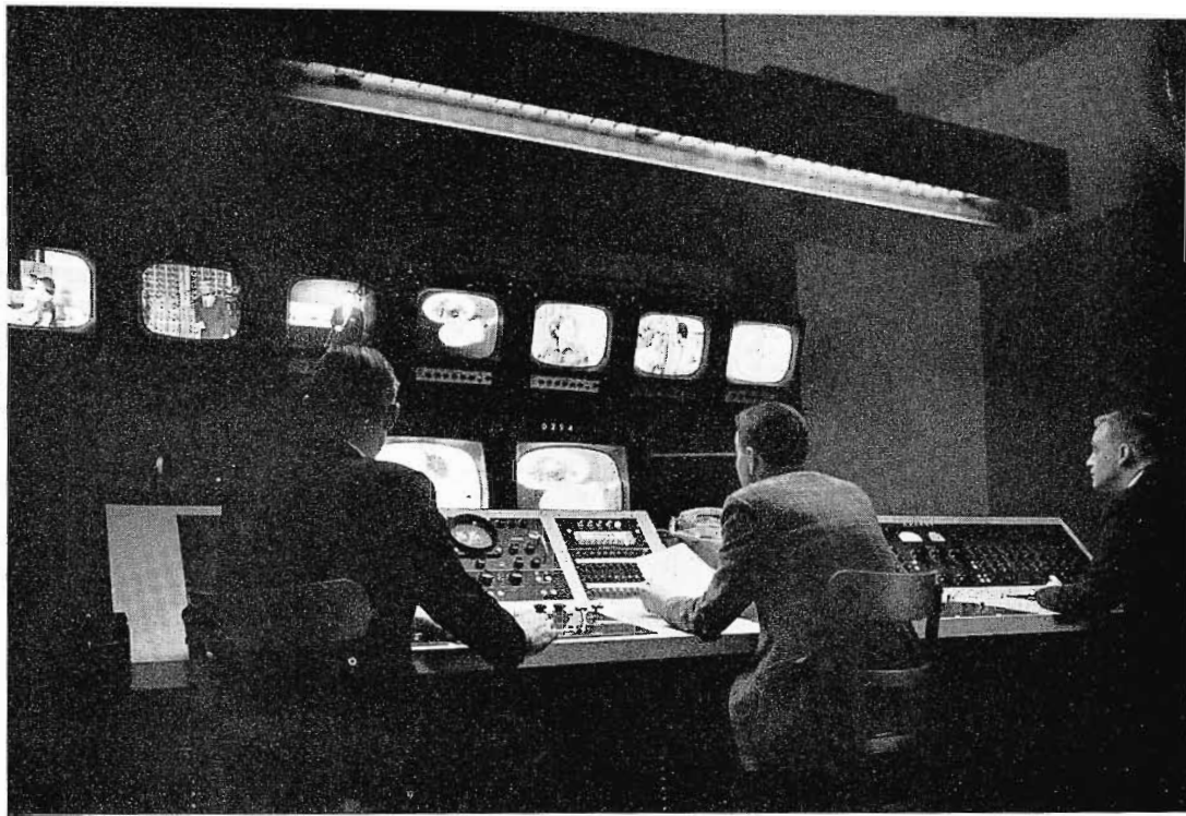
FIG. 8. Studio X—one of two mixing rooms showing input, preview and program monitors. The left side of the console is for video control, the right side for audio control. There are 9 video inputs, 18 audio channels. Dissolves and 150 RCA effects can be made here.
