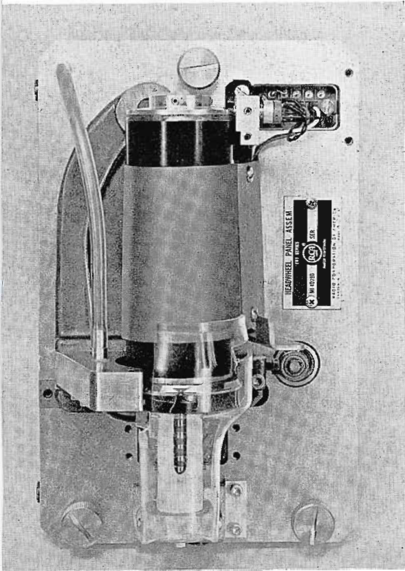
FIG. 1. Air bearing headwheel panel—available for use with all RCA tv tape recorders.
