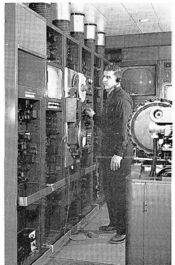
FIG. 42. KSTP has three color TV Tape Recorders—all type TRT-1B. Note exhaust ducts at top.
