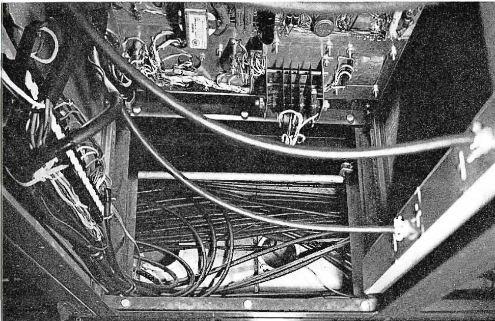
FIG. 30. At base of this rack note metal cellular flooring thru which cables enter trenches.
