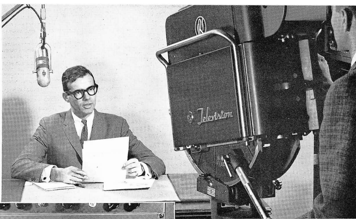
FIG. 20. Type TK-11 monochrome live camera at Reeves Studios is used for simple shots or commentary recordings in conjunction with location or studio recordings.
