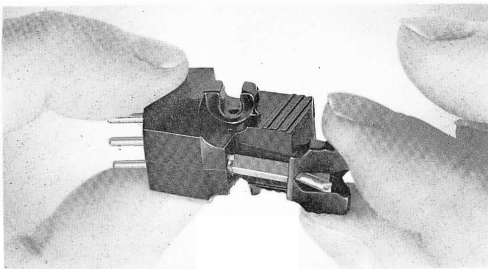
FIG. 1. Replaceable stylus construction eliminates the need for costly repairs in this new Universal Pickup Cartridge.
