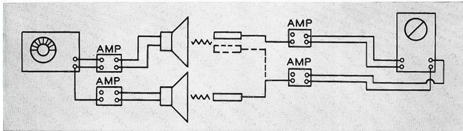
FIG. 5. Checking Loudspeakers.
