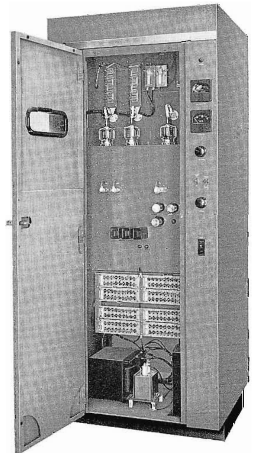
FIG. 2. Note uncrowded layout for ease of maintenance. Transformers on cabinet floor; silicon rectifiers immediately above; oscillator, IPA and audio amplifier in center; modulator and PA power tubes near top.
