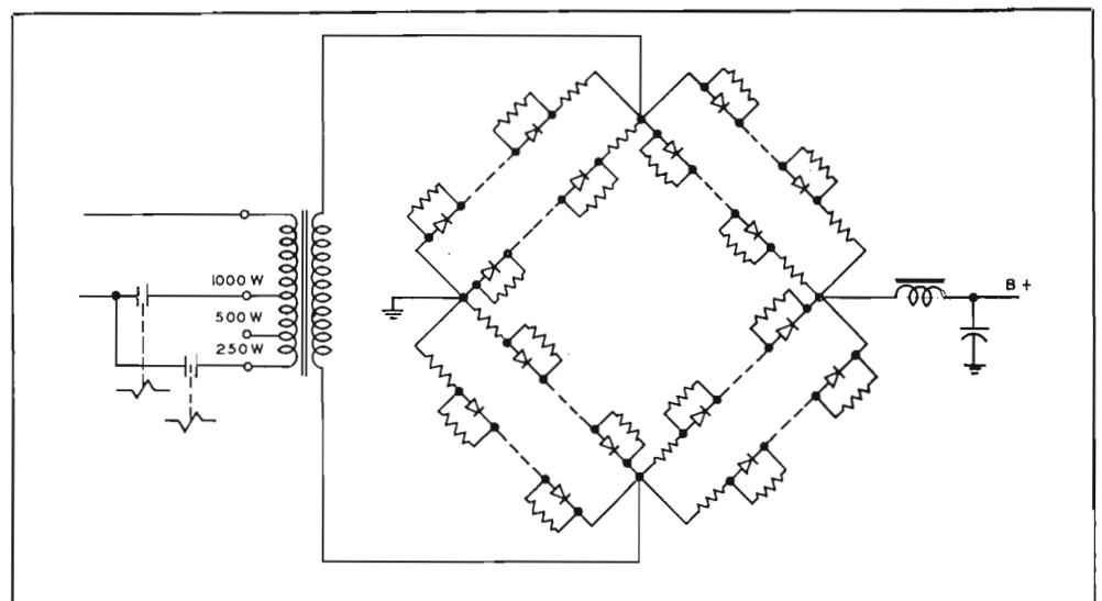
FIG. 4. Simplified schematic diagram of silicon-rectifier high-voltage power supply. Note series-parallel arrangement with voltage-sharing resistors, the series current-limiting resistors and the choke-input filter.
