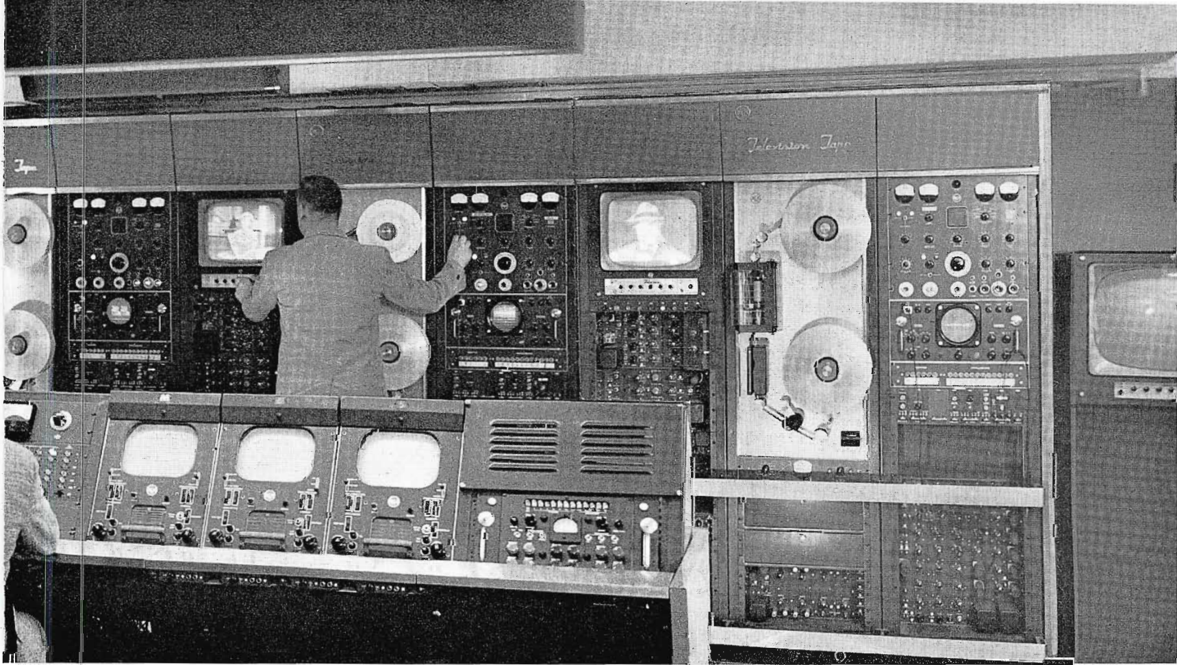
FIG. 1. Main Recording Room. This view shows six of the RCA television tape recorders and the camera control console.
