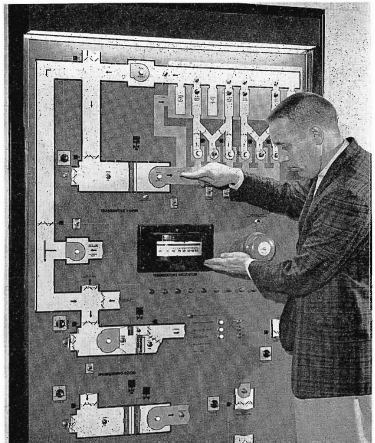
FIG. 35. George Merrill, transmitter supervisor, at air conditioning control panel. Three separate air conditioning systems are controlled from this panel. The top section controls transmitter and transmitter room. Colored lights indicate which blowers are operating and give warning of over temperatures. Temperatures of all critical transmitter points may be read on this control board.
