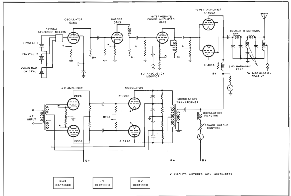
FIG. 3. Simplified circuit schematic, BTA-1R1. Note that only one power-tube type is used; only nine tubes in entire transmitter . . . of only five types.
