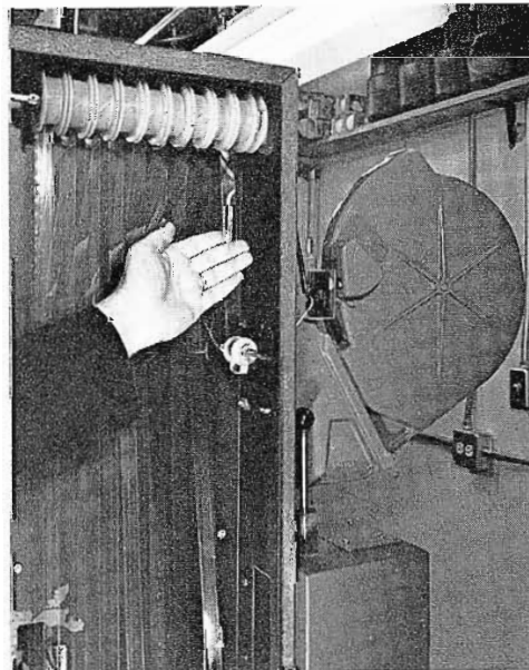
FIG. 59. Special devices added by KSTP to color processor so that film cannot jump off roller; also note micro-switch to indicate low film supply.
