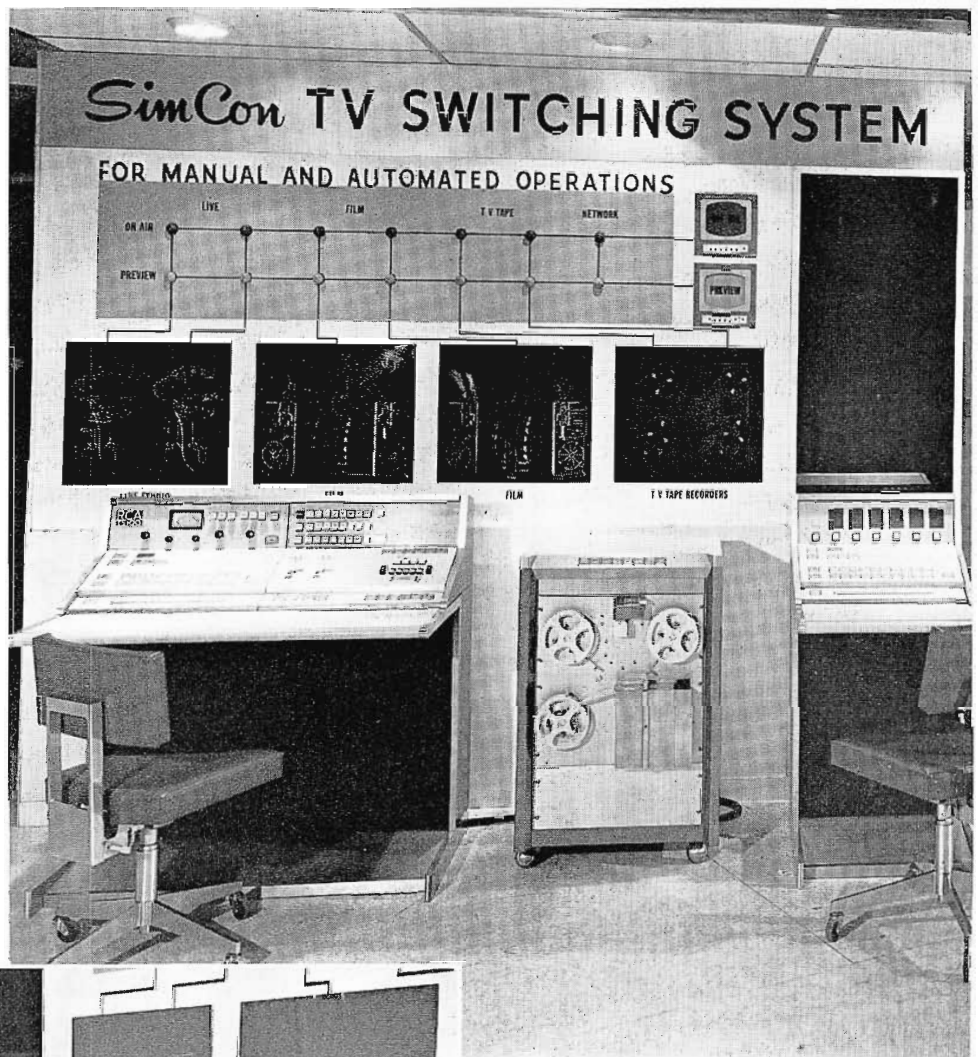
FIG. 5. TV's new control console handles all the station's switching operations, controls associated mechanical equipment, and can be completely automated by adding clock and memory units.
