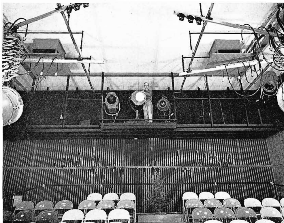
FIG. 13. Audience end of Studio 3. Catwalk at rear can be used to support color TV camera as well as follow-spots and dimmers.
