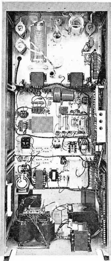
FIG. 6. Rear view. Note clear accessibility to all components. Laced wiring harnesses and screw-type terminal strips make for easy maintenance.
