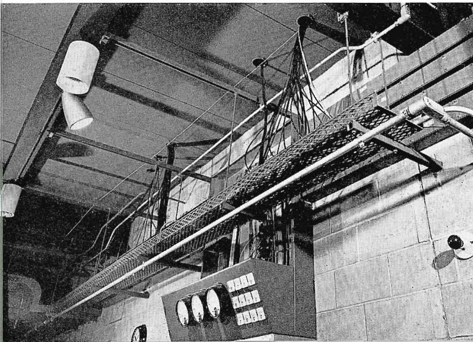
FIG. 31. A view of the basket construction used beneath the cellular floor in the engineering area to transport cables to other portions of the building.
