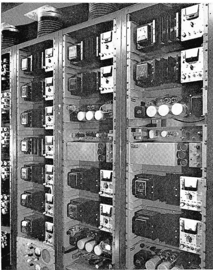
FIG. 36. Power racks showing 15 WP-16 solid-state power supplies for color cameras, terminal equipment, switchers, etc. The low heat dissipation of these power supplies permits loading up a rack with power without worrying about overheating.
