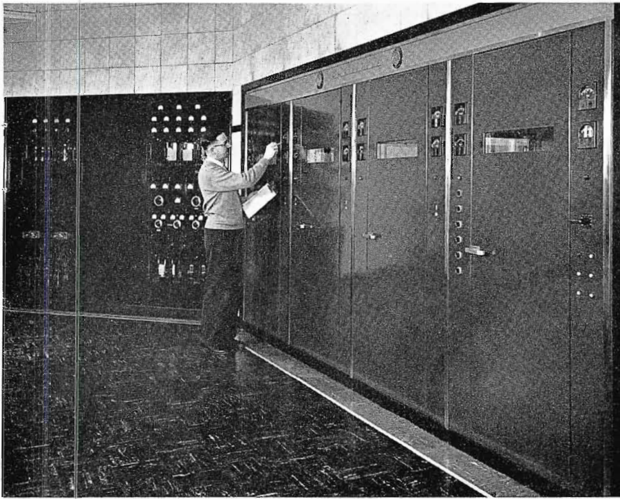
FIG. 65. AM Transmitter supervisor, Howard Carlson, at RCA 50-kw Ampliphase transmitter. At left is 1-kw auxiliary transmitter.
