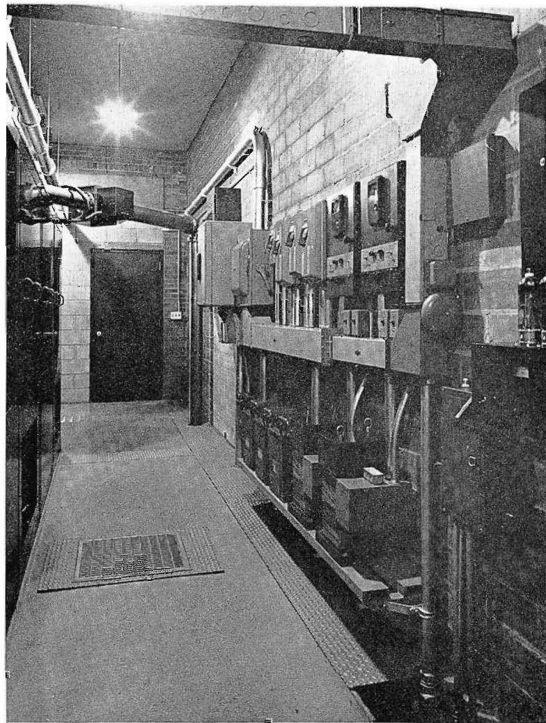
FIG. 66. Note neat and compact arrangement of power and control equipment for 50-kw ampliphase transmitter.
