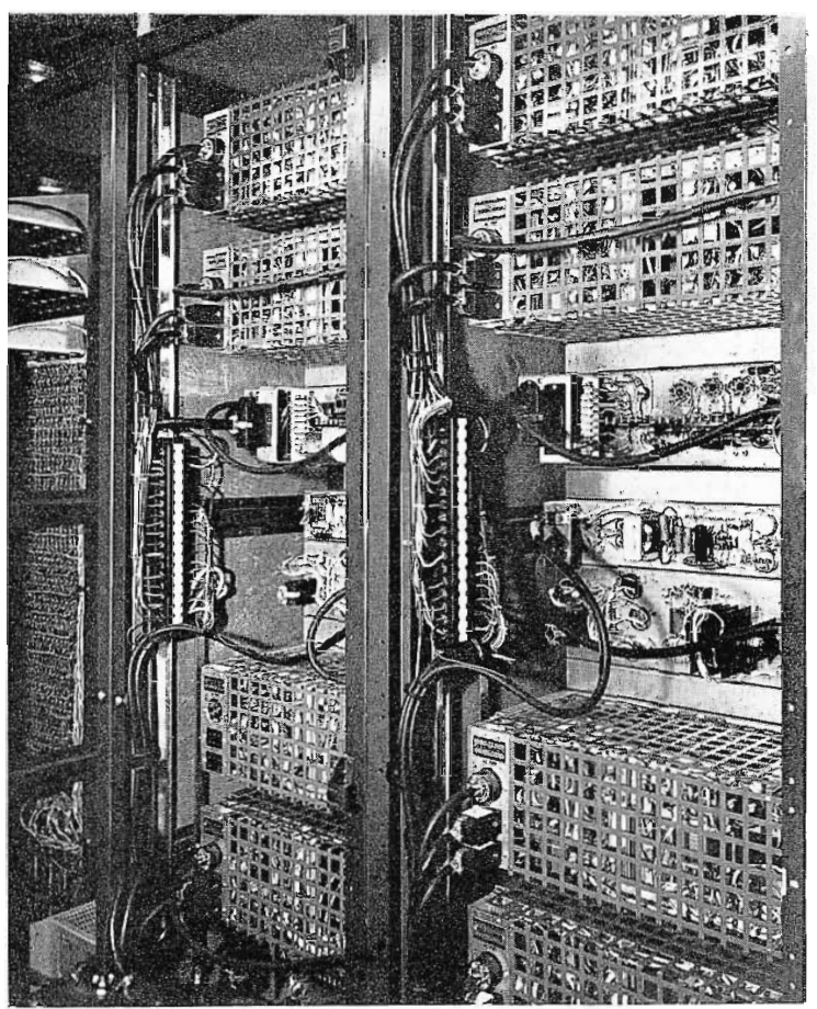
FIG. 37. Backs of racks in power supply section. Note on left of each rack a large terminal block. These provide power distribution to the various services. These blocks are sectionalized and individual sections can be taken out or replaced at a moment's notice.
