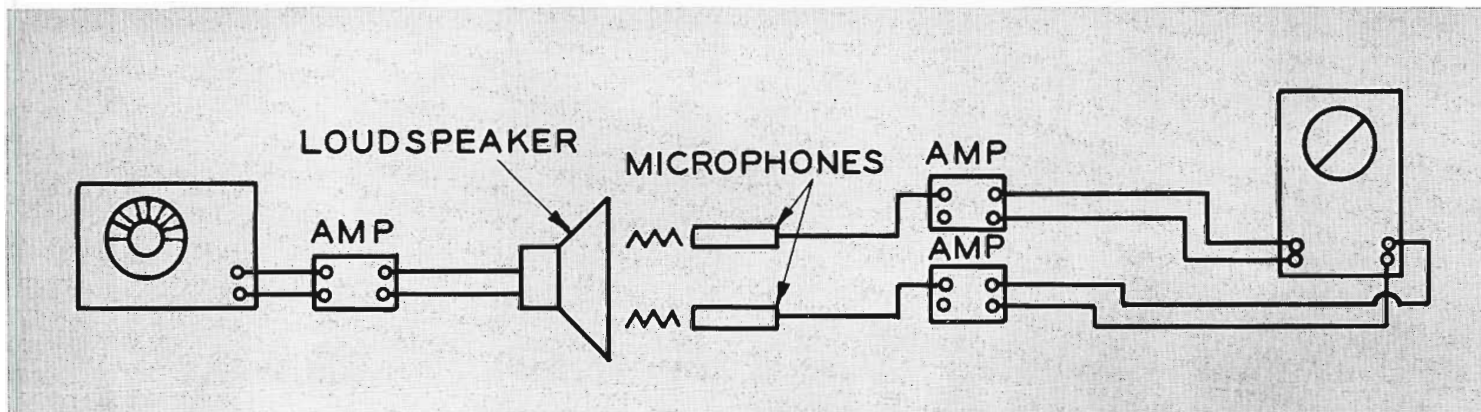
FIG. 4. Checking Microphones.
