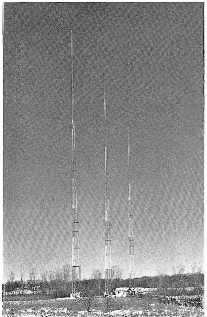
FIG. 68. KSTP beams power westward at night, is non-directional in daytime. First tower is 340 feet high and is top loaded. Second tower is also 340 feet high while third is 296 feet high.
