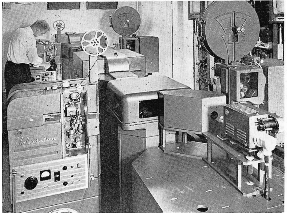
FIG. 12. Telecine room equipped with two TP-15 multiplexer nests with TK-21, TK-26 Film Cameras and TP-35, TP-16 TV Film Projector equipments.
