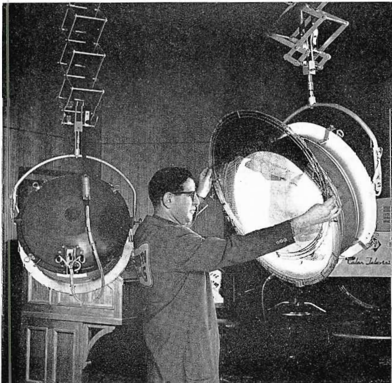
FIG. 17. Mobile rail system is employed for supporting and positioning of lighting fixtures. Note air-conditioning diffusers. Also part of ceiling is plastered for "live" acoustical effects.
