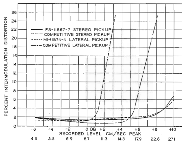
FIG. 2. Lateral intermodulation distortion vs recorded level, RCA 12-5-39 Record.
