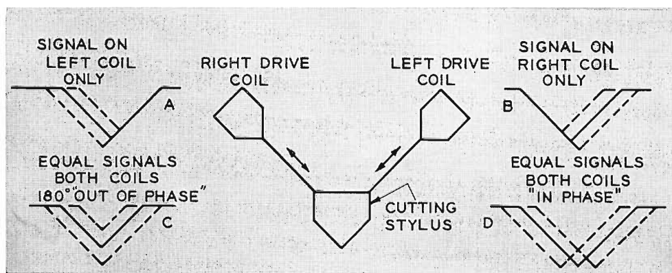
FIG. 1. 45°-45° Stereo Disc Recorder.
