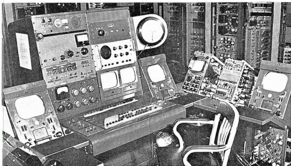
FIG. 3. Station-built console housing incorporates TS-40 with room for expansion.
