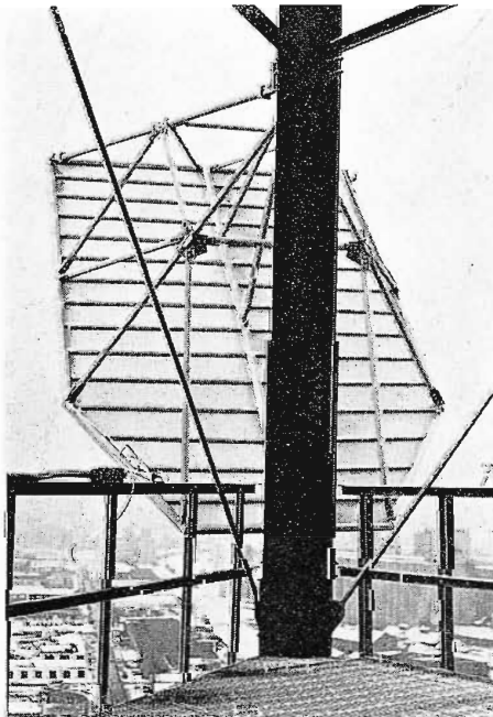
FIG. 46. Passive reflector is mounted at 250-foot level of KSTP tower.
