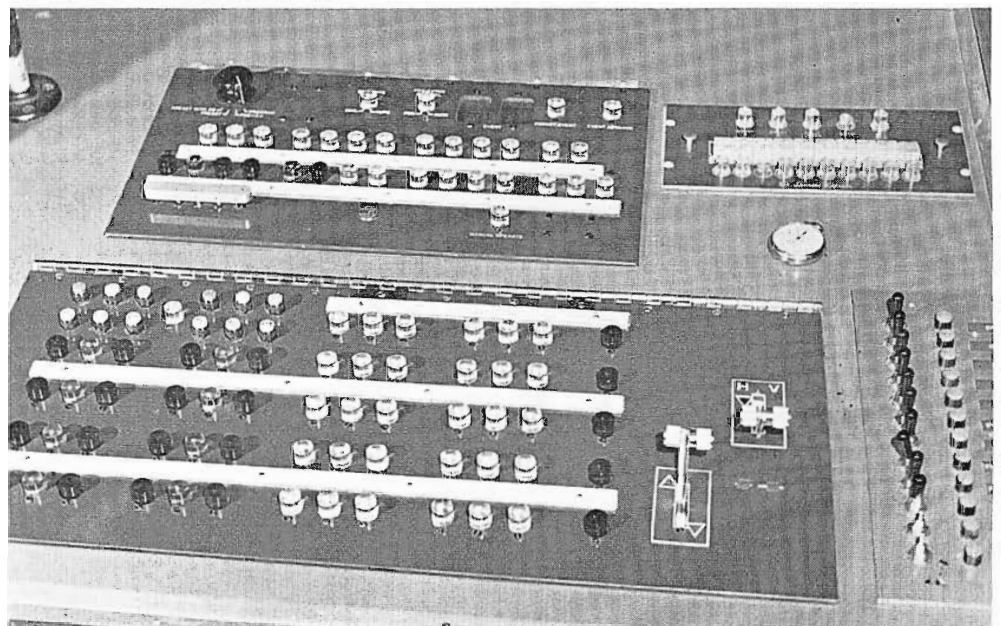
FIG. 8. One of the KBTV TS-40 systems. Top left, TSA-1 Control Panel; top right TG-25 Special Effects Selection; lower right, TS-40 Director's Panel; and lower left, Intercom Control.
