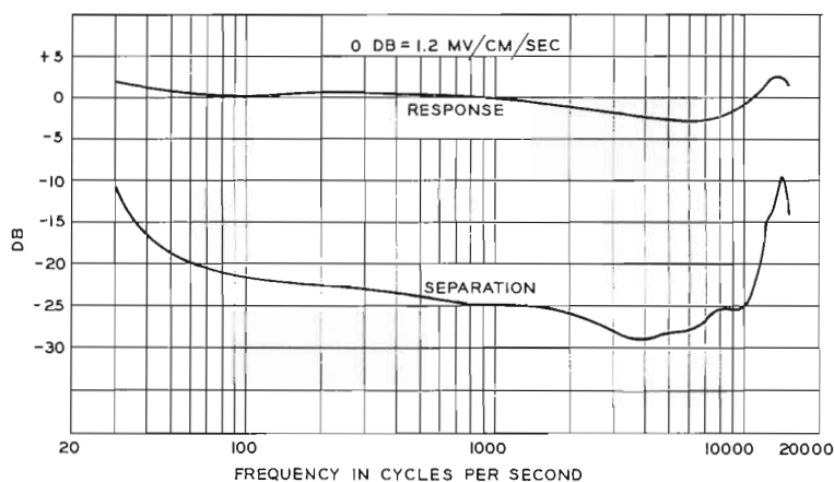
FIG. 3. Frequency response and channel separation, Westrex 1-A Record.
