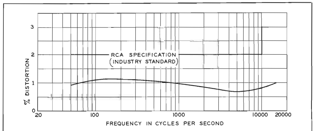
FIG. 5. Typical distortion vs. frequency curve. Note that distortion at maximum is only slightly more than half of the industry-standard specification.
