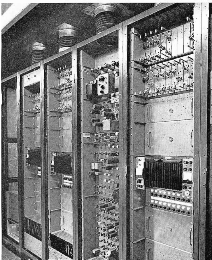
FIG. 34. TS-40 Switching Arrangement. On far left is master control TS-40. Next is TS-40 switcher and TG-25 special effects generator for control room 3. Right rack is TS-40 for control room 2. Note air exhaust ducts at top of racks.
