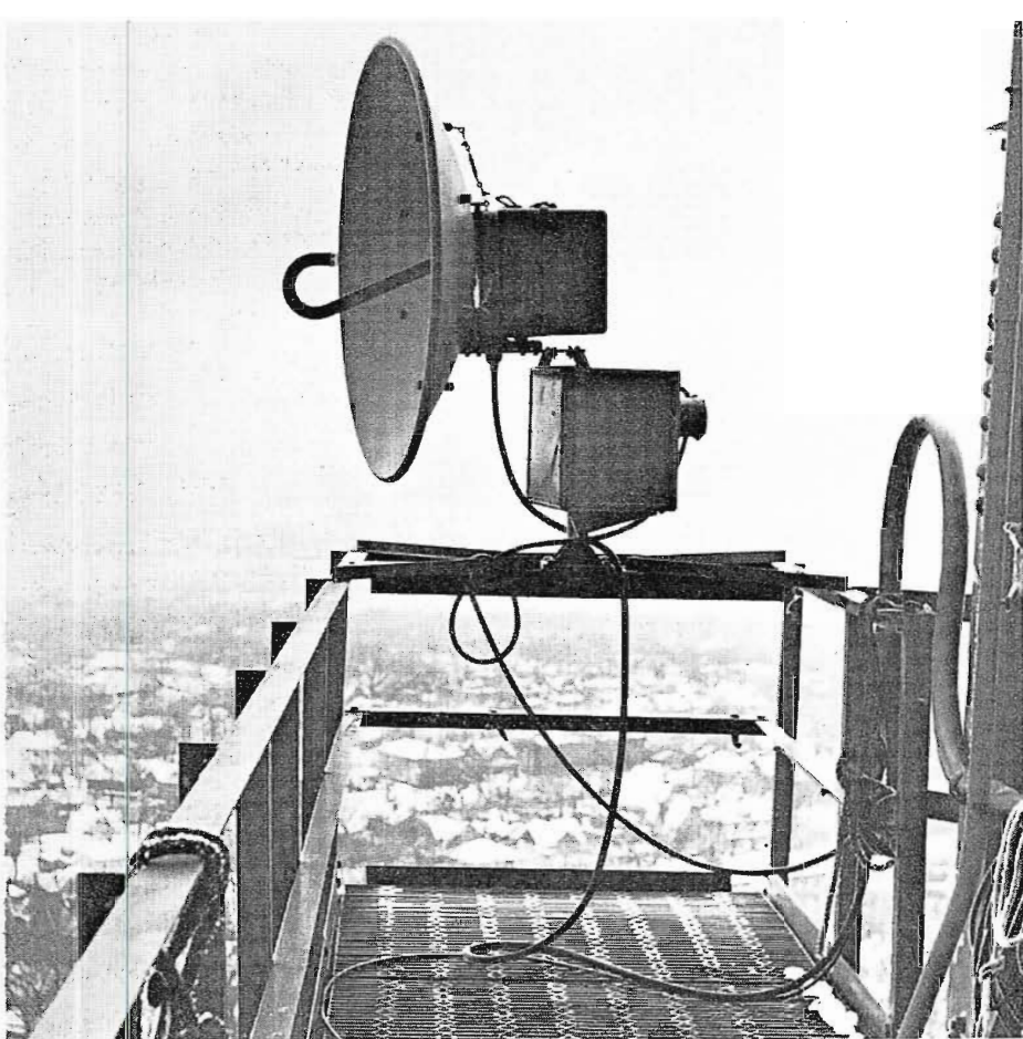
FIG. 43. Tower-mounted microwave receiver and parabola at KSTP for link with remote cruiser. Note remote positioning unit for aligning parabola.
