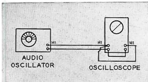
FIG. 2. Phase Indicator.
