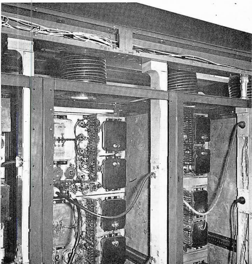
FIG. 38. Top of power supply racks. All A-C wiring for racks is carried overhead in 4-inch square ducts and is then carried downward inside the rack in wire mold to insure complete separation of power, video, and audio wiring.
