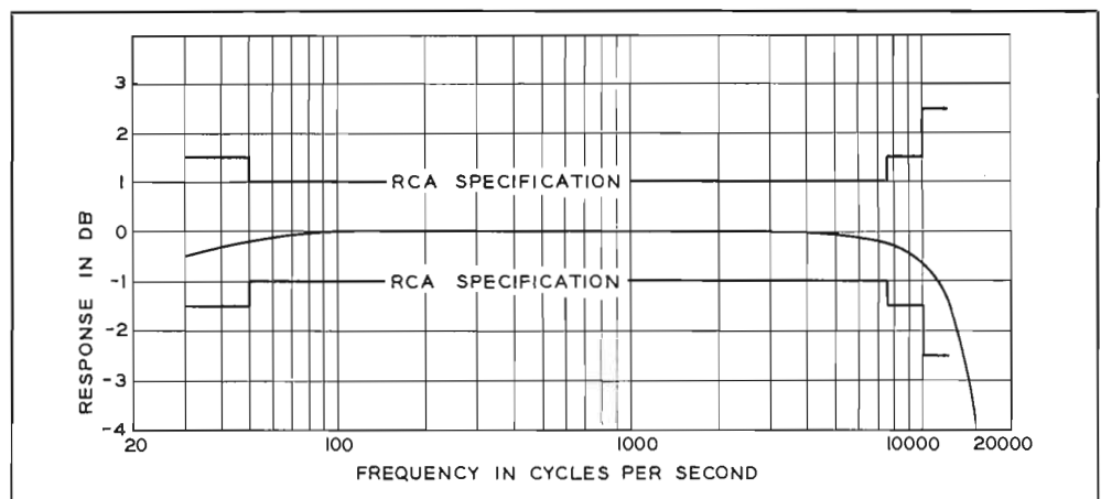
FIG. 7. Typical frequency-response characteristic, BTA-1R1. Note that response is well within RCA specifications and these are well within industry standards. Note also the smooth roll-off to 30 cps and 10 kc. Truly, high-fidelity AM "sound".
