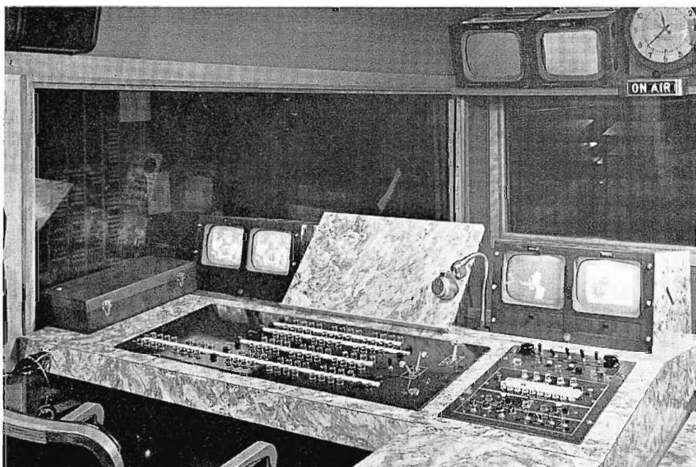
FIG. 6. KTBS custom console, as designed by the author, accommodates TS-40 controls, special effects selection and remote control of tape recorder and projectors.
