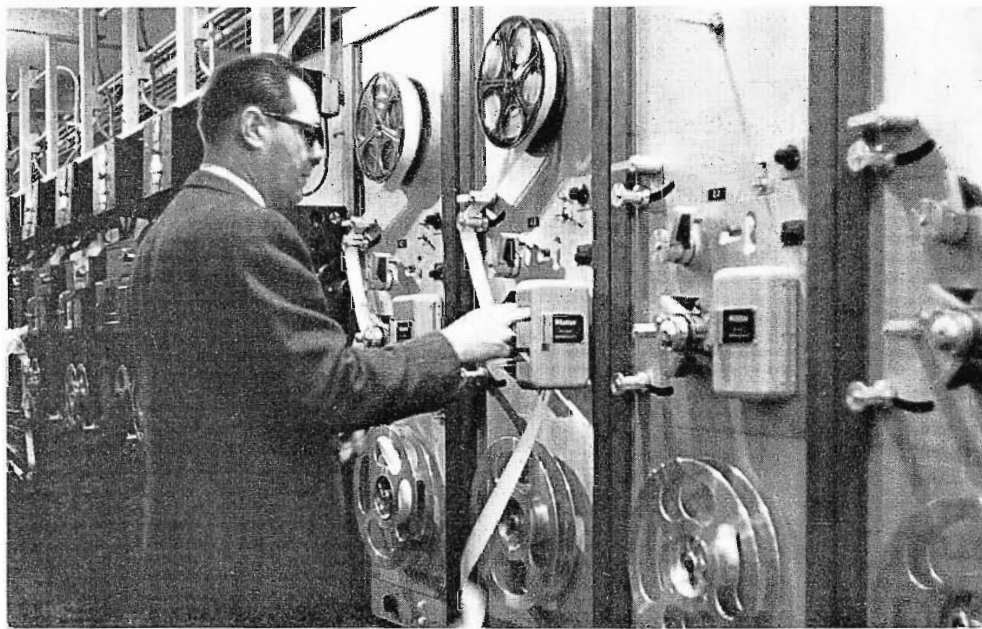
FIG. 13. Sound dubber room, showing several of 40 sound playback machines, which use sprocketed magnetic or optical film. Richard Vorisek loading dubber.
