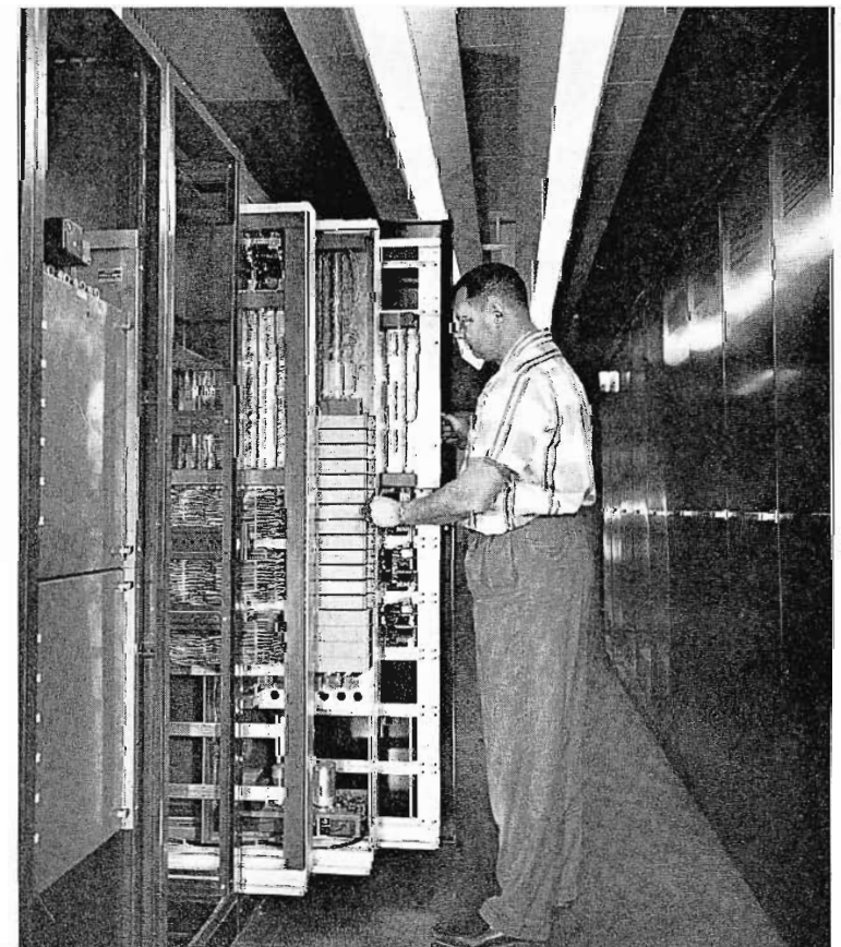
FIG. 28. Rack equipment for automation system is designed for convenient installation and ease of maintenance. Three double sided units are mounted on rollers, making every component and connection conveniently available for testing and servicing. John Reinke, technician, demonstrates sliding action.
