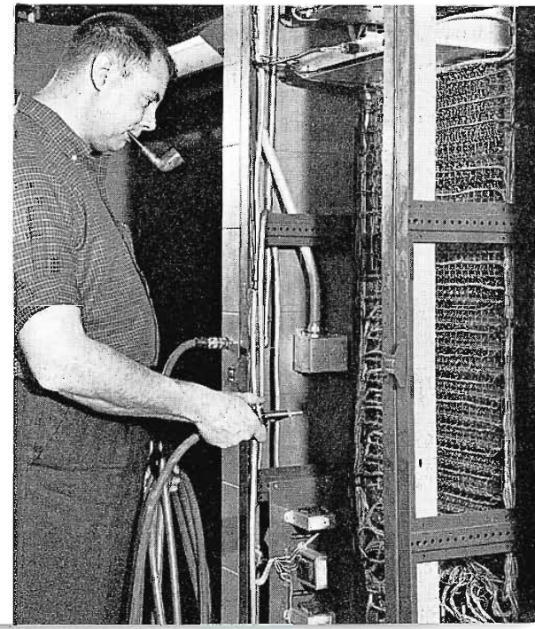
FIG. 32. John Reinke using air connection at end bell of rack section. These air outlets provide air from 2 to 100 pounds through a regulator to simplify cleaning of the rack equipment. . . . Also shown is part of relay bank of production intercom system. This provides 20 stations which can be operated in two ways: Individual selection, unit to unit; or public address selection. Up to 19 stations can be tied together and operated by a master switch.
