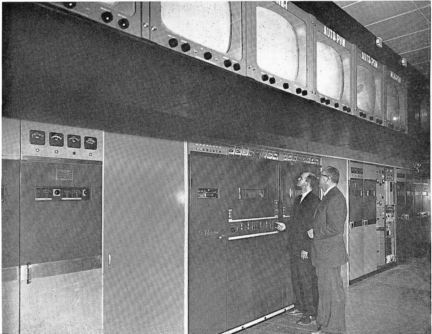
FIG. 22. Type TT-25CL 25-kw main TV transmitter. Fred Street, director of operations, and Larry Larson, director of research and development. At right TT-2AL 2-kw auxiliary TV transmitter. Coax switches permit either transmitter to be connected to one of two antenna systems.
