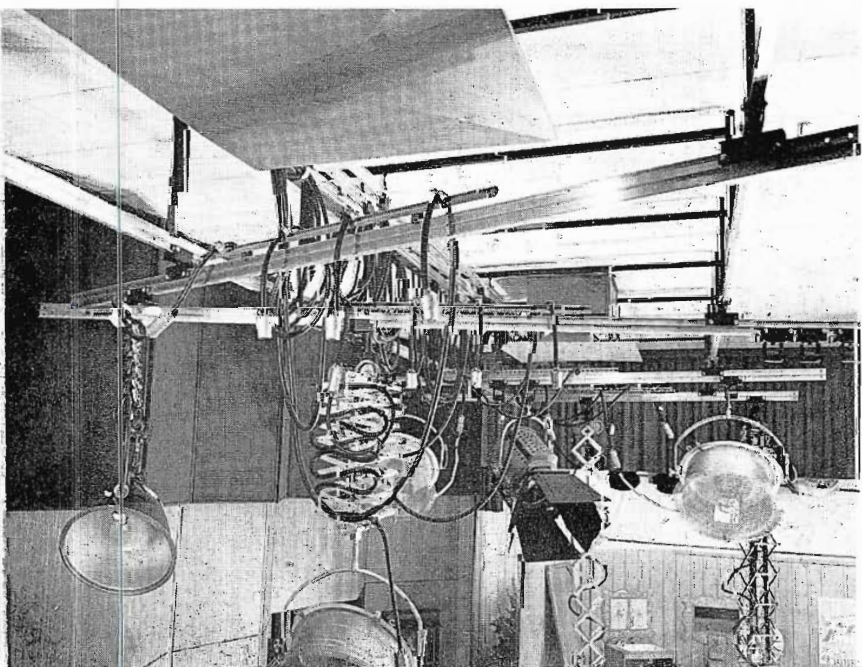
FIG. 17. Mobile rail system is employed for supporting and positioning of lighting fixtures. Note air-conditioning diffusers. Also part of ceiling is plastered for "live" acoustical effects.
