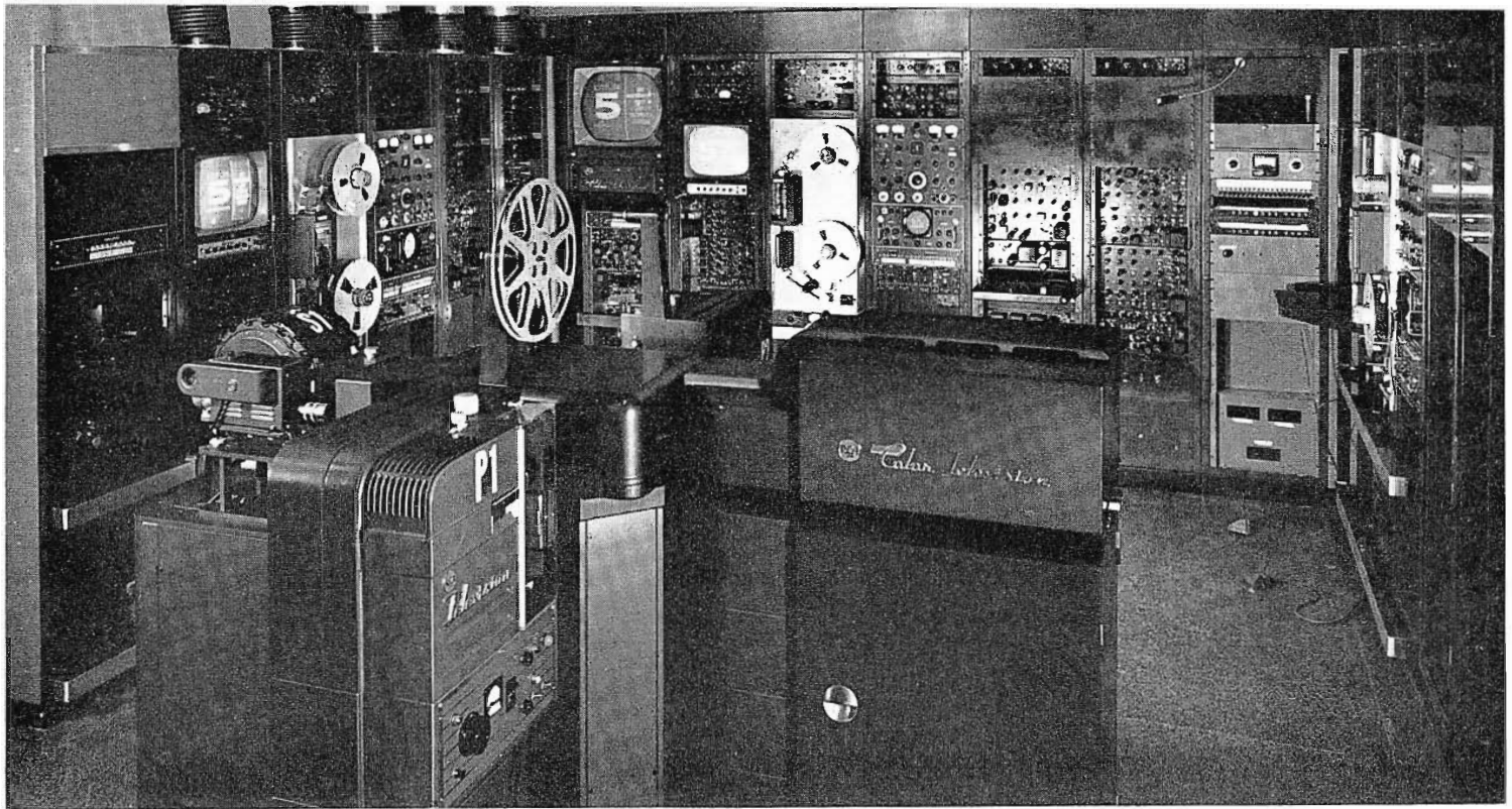
FIG. 21. In foreground is color TV film island. (There is also a monochrome film island.) Three TV Tape recorders are shown in U-shape background. All three are color recorders.
