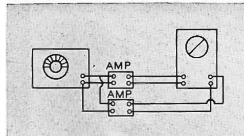
FIG. 3. Checking Amplifiers.
