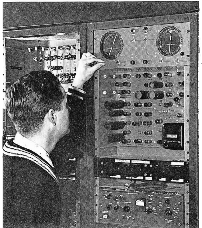
FIG. 44. Transmitter technician, Clint Barstad, adjusting elevation control of parabola on 250-foot level of tower. Control at right is used for azimuth.
