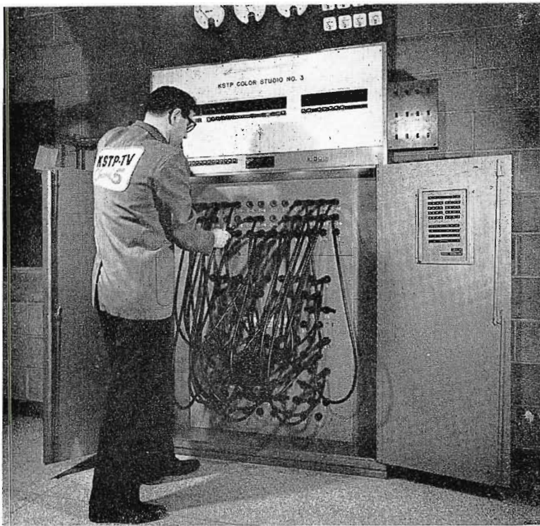
FIG. 14. (left) Three meters at top are load current indicators for the 3 phases on the 24 non-dim 50-amp circuits. Group of 12 meters and outboard panel are metering and control for 12 dimmer 50-amp circuits. All dim and non-dim circuits appear at top part of patch panel, while the 85 load circuits appear in lower part.
